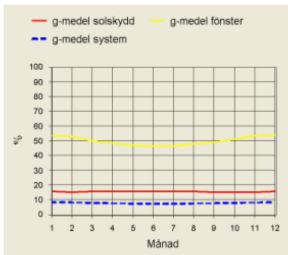
Figur 1 g-verdi Orion Climaflex
